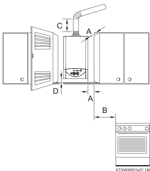
Fig. 7 Distances minimales
