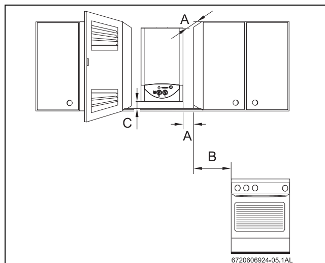
Fig. 7 Distances minimales
